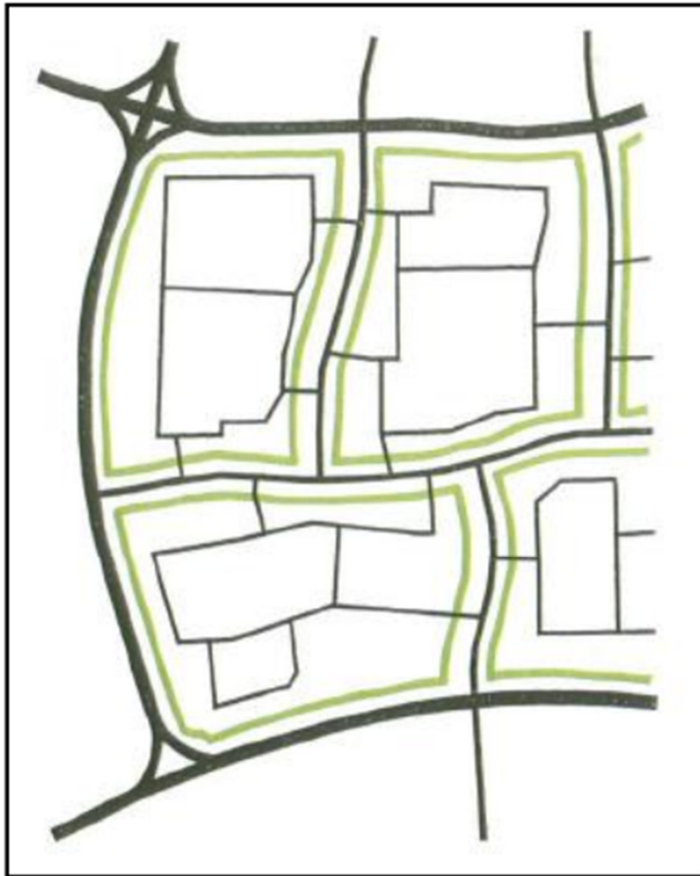
Figure 2.4 Hierarchy of distributors and cellular structure
